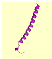
alpha helix
